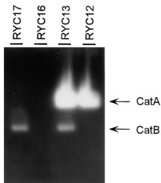
Figure 3. Catalase activity assay. Protein extracts from conidia of wild-type (RYC13), catA (RYC17), catB (RYC12), and catA/catB (RYC16) mutants were fractionated in native polyacrylamide gels and stained for catalase activity.
