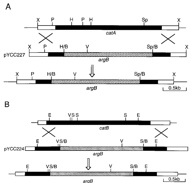
Figure 1. Deletion of catalase genes. (A) Plasmid pYCC227 was constructed by replacing a major portion of the catA coding region (black box) with the argB gene (hatched box). Linearized pYCC227 was used to transform the argB -deleted strain RMS011. The catA -deleted transformants were screened by PCR and confirmed by Southern blot analysis. (B) Plasmid pYCC224 was constructed by replacing nearly 50% of the catB coding region (black box) with the argB gene (hatched box). The catB -deleted transformants were screened as in the catA deletion. B, BamHI; E, EagI; V, EcoRV; H, HpaI; P, PstI; S, StyI; Sp, SphI; X, XbaI.
